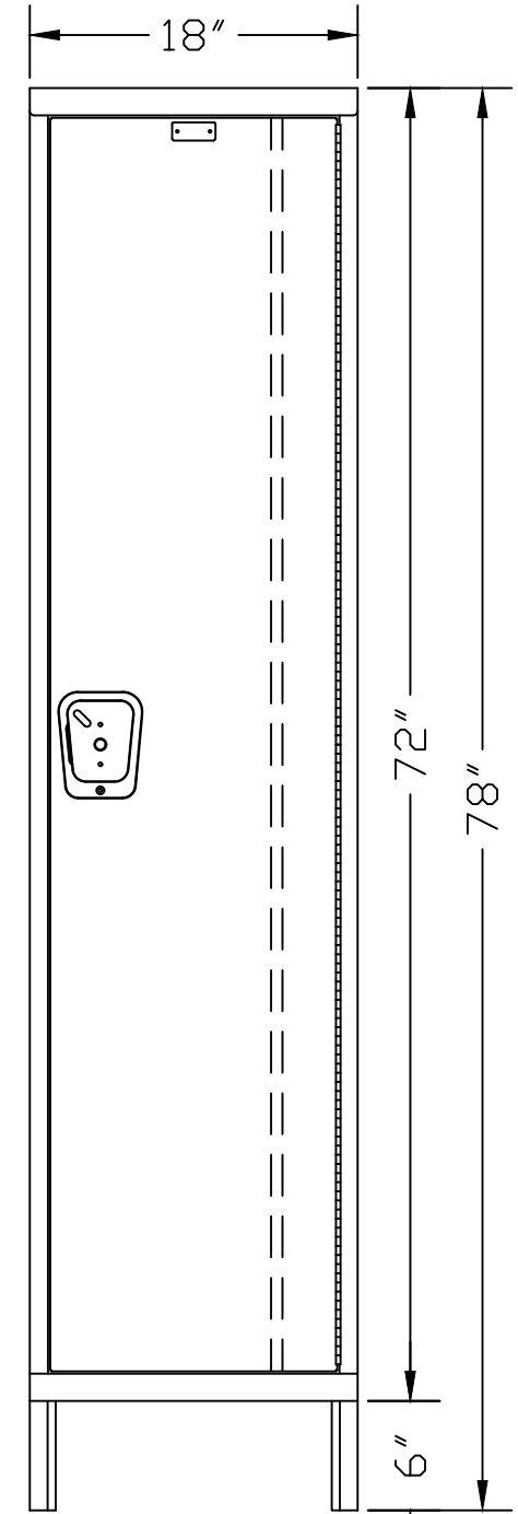
FRONT VIEW
