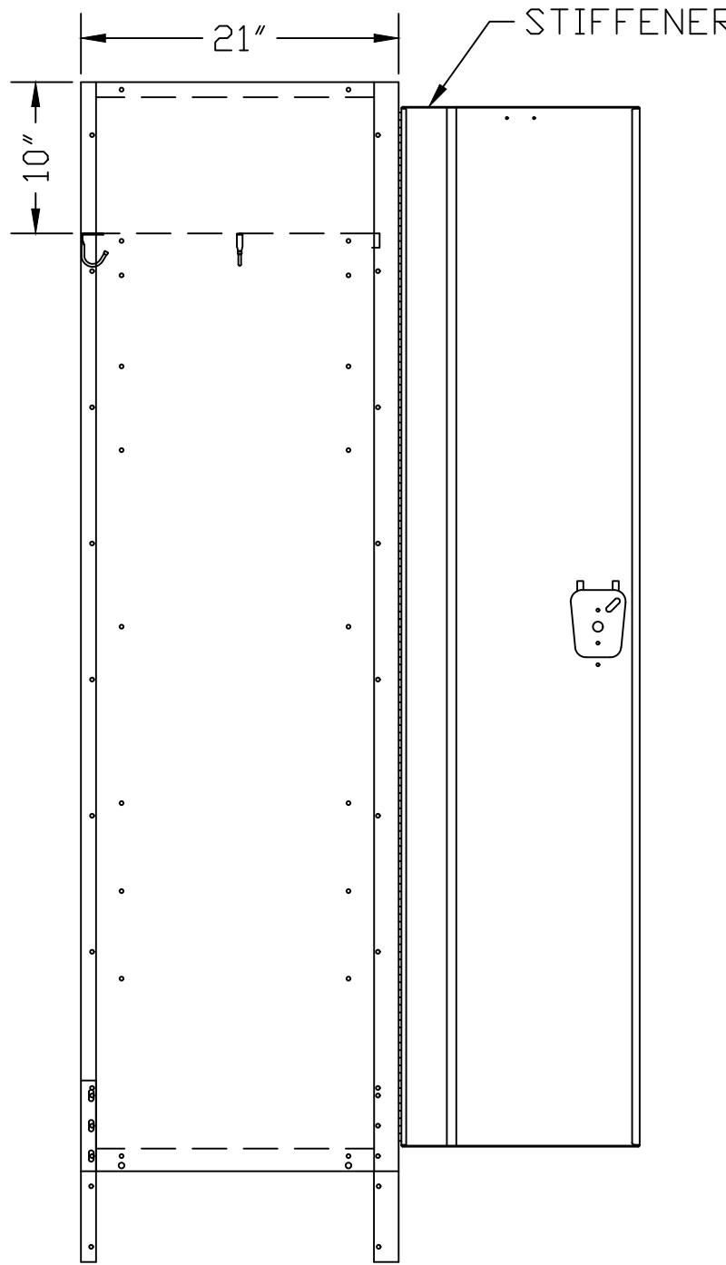
SIDE VIEW
