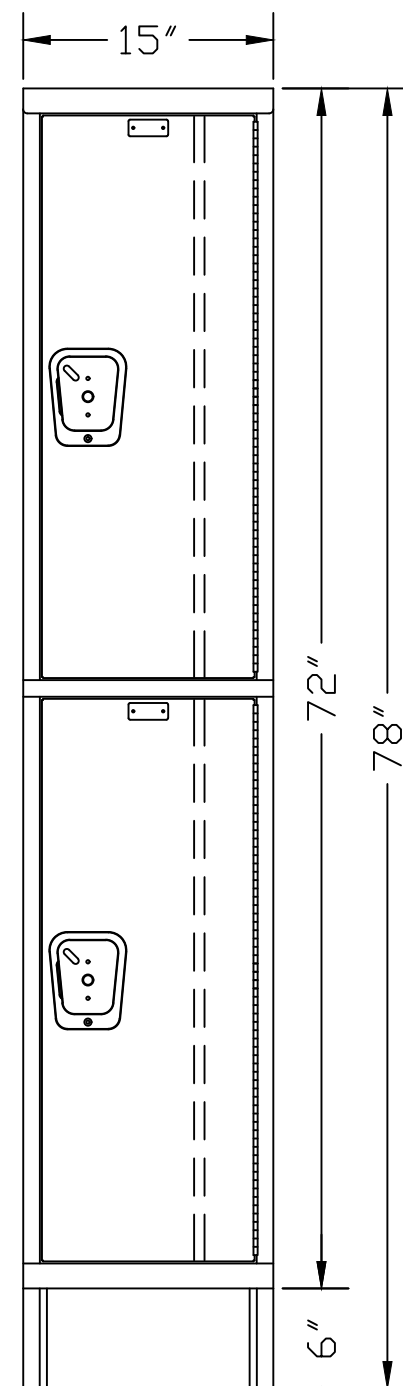
FRONT VIEW
