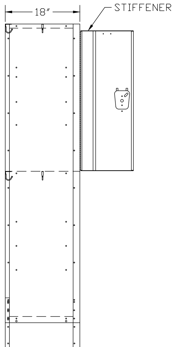
SIDE VIEW
