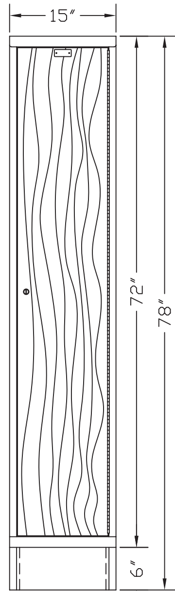
FRONT VIEW 1-WIDE
