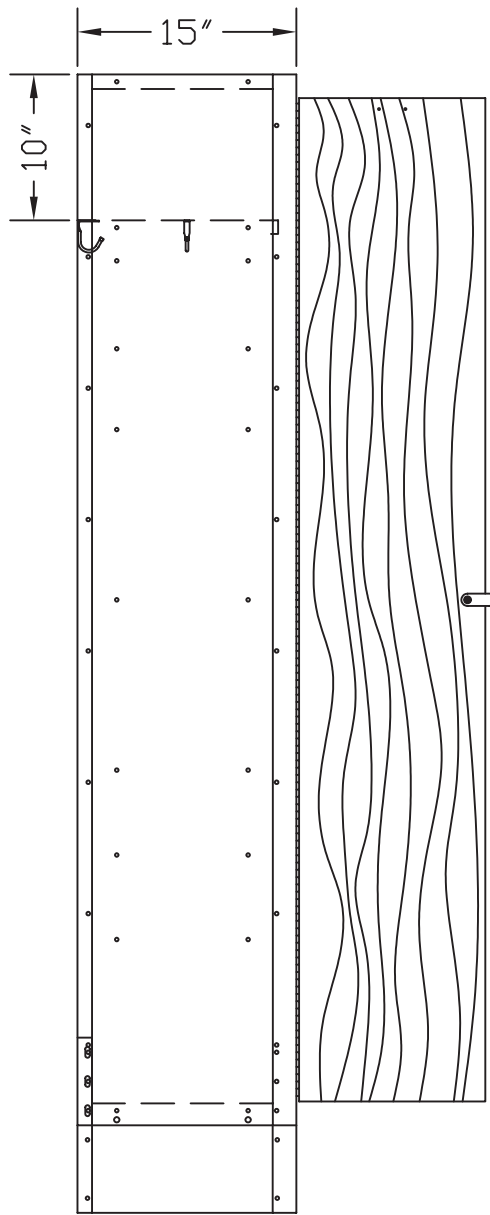
SIDE VIEW
