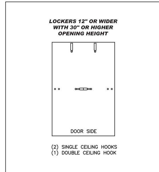
HOOK CONFIGURATION
