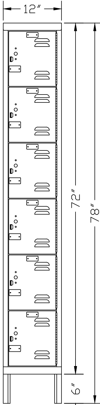
FRONT VIEW
