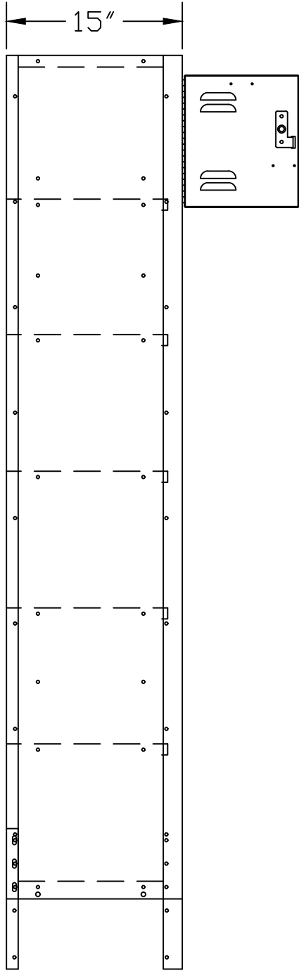
SIDE VIEW
