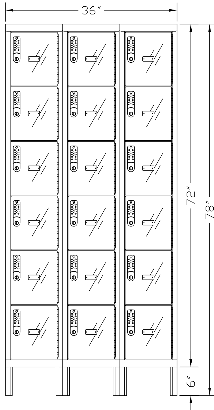
FRONT VIEW
