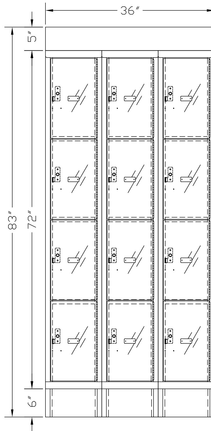
FRONT VIEW
