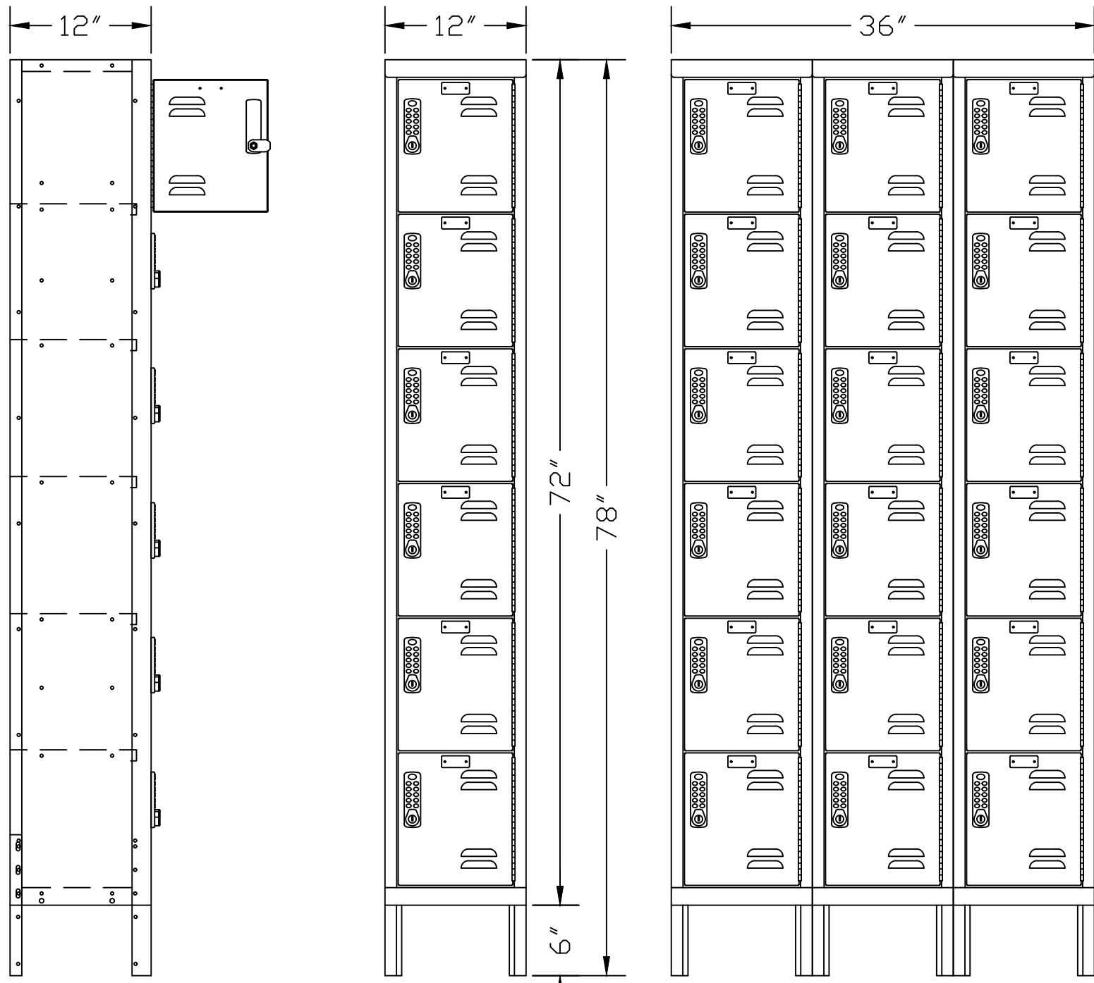
SIDE VIEW
