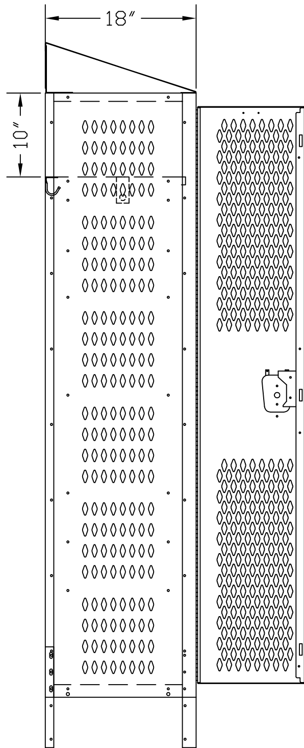
SIDE VIEW
