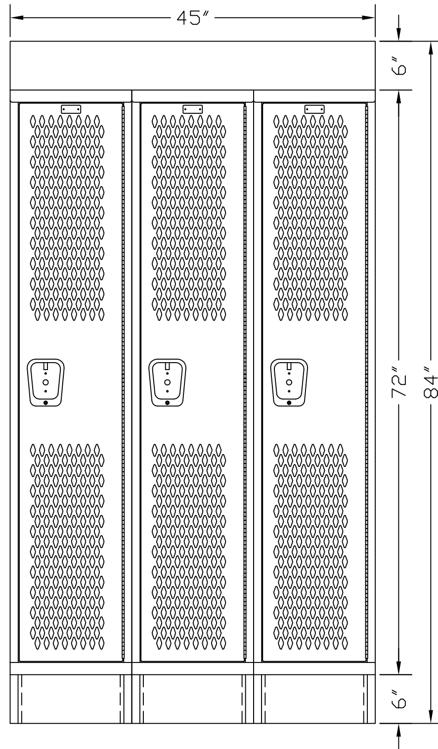
FRONT VIEW
