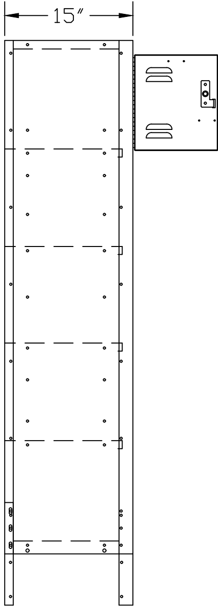
SIDE VIEW
