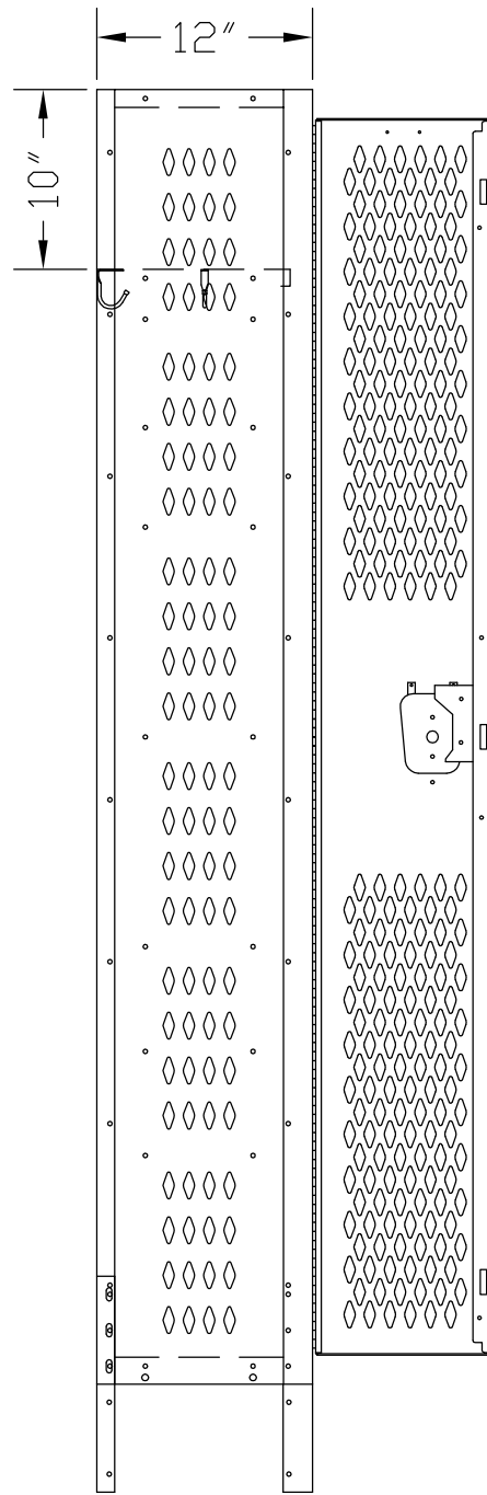
SIDE VIEW
