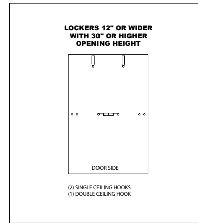
HOOK CONFIGURATION
